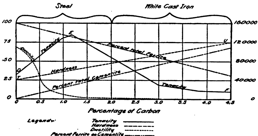
Fig. 59. Physical Properties and Assumed Microscopic Constitution of the Pearlite Series, Graphiteless Steel Slowly Cooled, and White Cast Iron.
